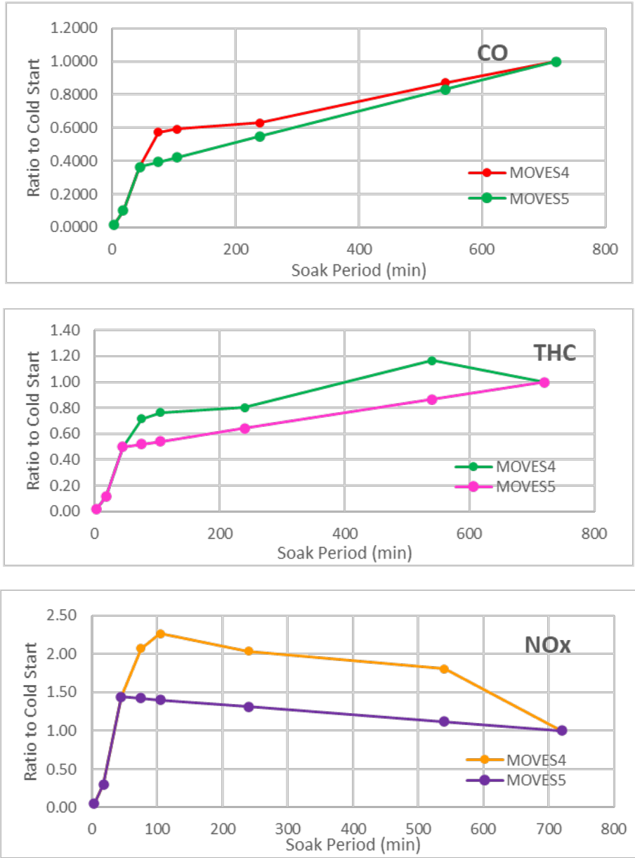
Figure 3-139 Modification of intermediate soak rates comparing the ratio to cold start for MOVES4 and for the version incorporating LMDV (MOVES5)
