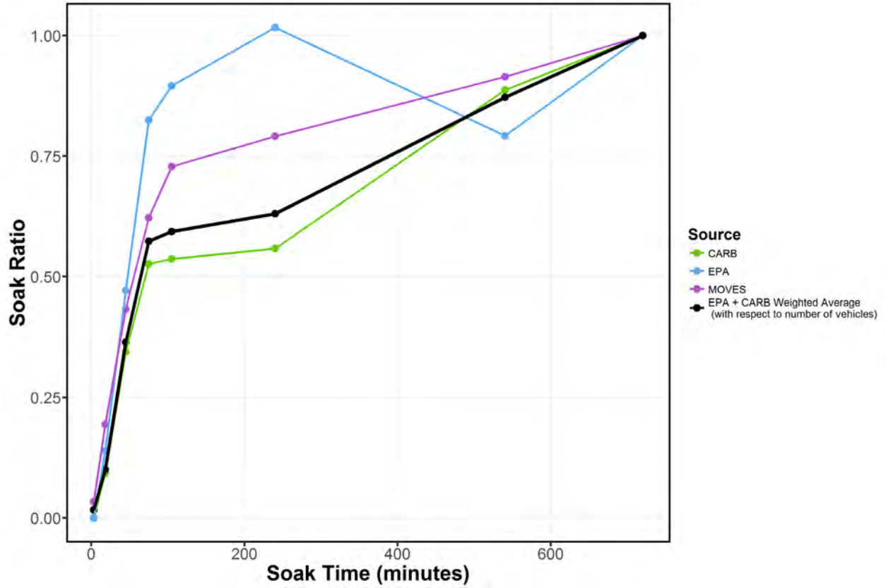
Figure 3-91 CO: Program-specific and final soak-time ratios for Tier-2/LEV-II vehicles. The “MOVES” line represents the values in MOVES for MY 2004 and later
