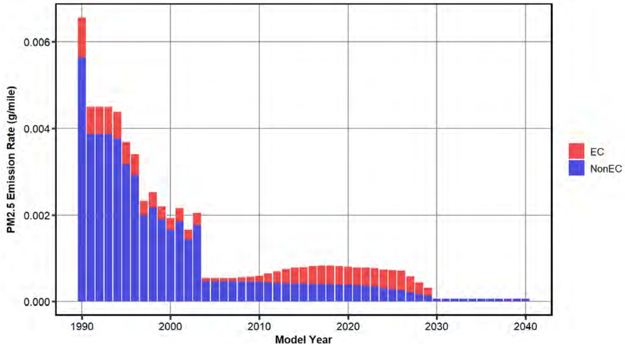
Figure 4-34 EC and NonEC PM2.5 emission rates for age 0-3 passenger cars averaged across a nationally representative operating mode distribution
