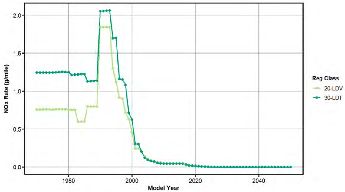
Figure 3-142 Base running emission rates for NO x from age 0-3 gasoline light-duty vehicles averaged over a nationally representative operating mode distribution
