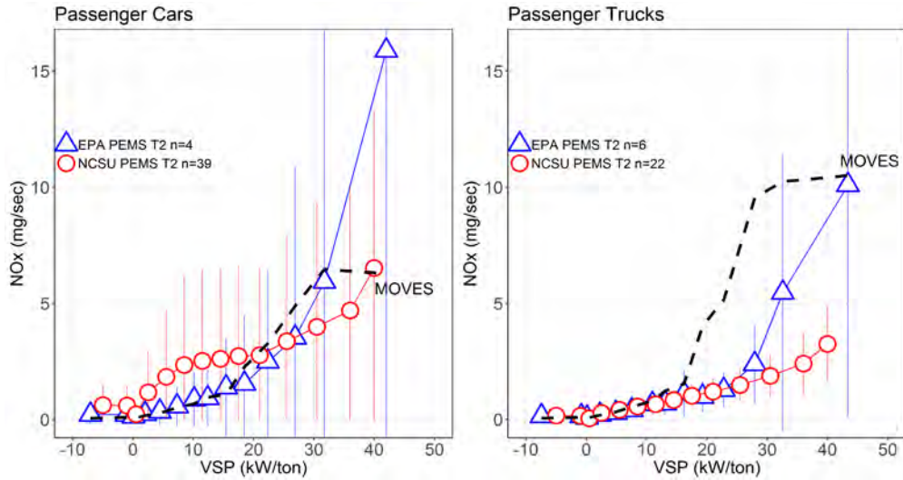
Figure 3-28 Trends in NO x emissions for passenger cars and trucks, as measured by two PEMS instruments and as represented in MOVES2014 emission rates.
