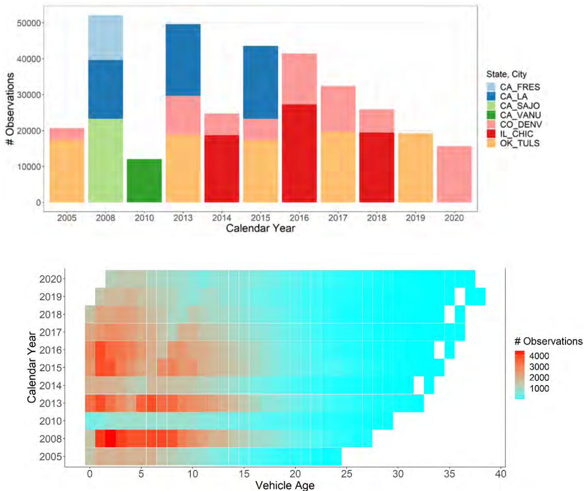
Figure 6-1. Top panel: Number of Vehicle Ammonia Measurements by Location and Calendar Year. Bottom panel: Number of Vehicle Ammonia Measurements by Vehicle Age and Calendar Year
