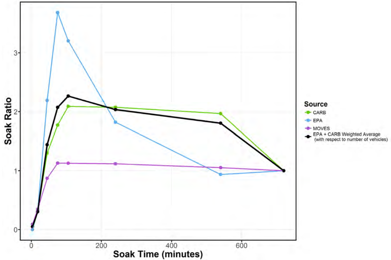
Figure 3-92 NO x : Program-specific and final soak-time ratios for Tier-2/LEV-II vehicles. The “MOVES” line represents the values in MOVES for MY 2004 and later
