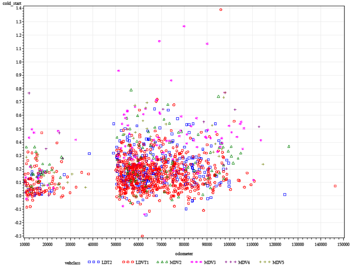
Figure 3-97 Cold-start FTP emissions for NO x (g) vs. odometer (mi), for LEV and ULEV vehicles, from the IUPV program
