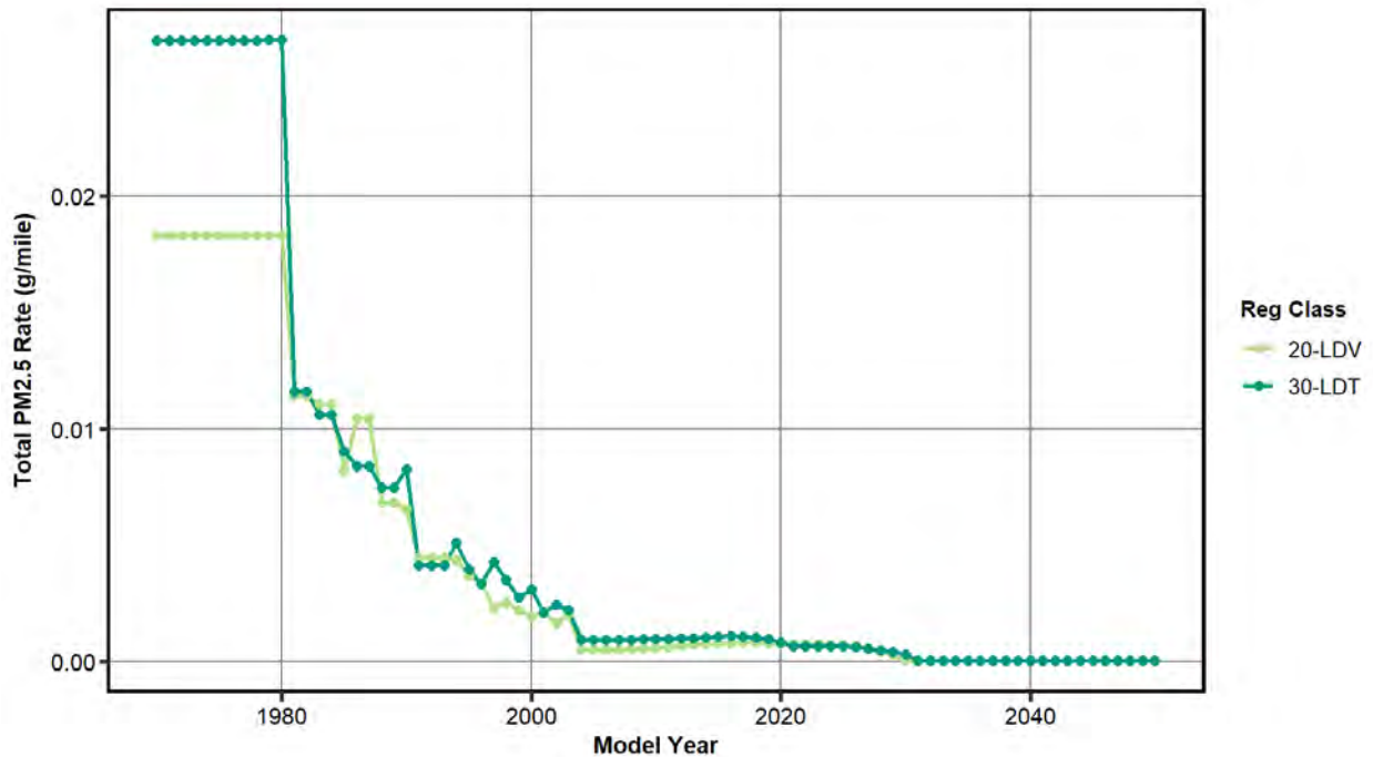
Figure 4-33 Base PM2.5 running emission rates for age 0-3 gasoline light-duty vehicles and light-duty trucks averaged using nationally representative operating mode distributions
