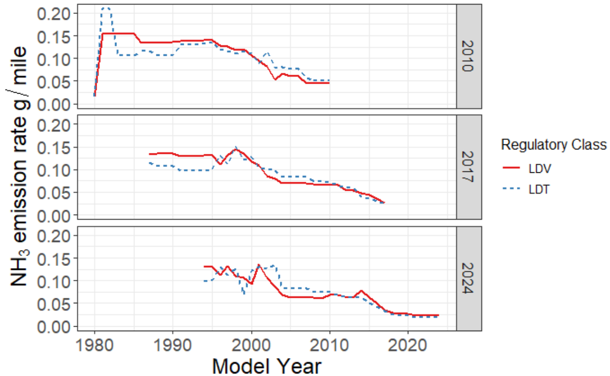
Figure 6-7. MOVES NH 3 emission rates (g/mile) by model year, regulatory class for calendar years 2010, 2017 and 2024
