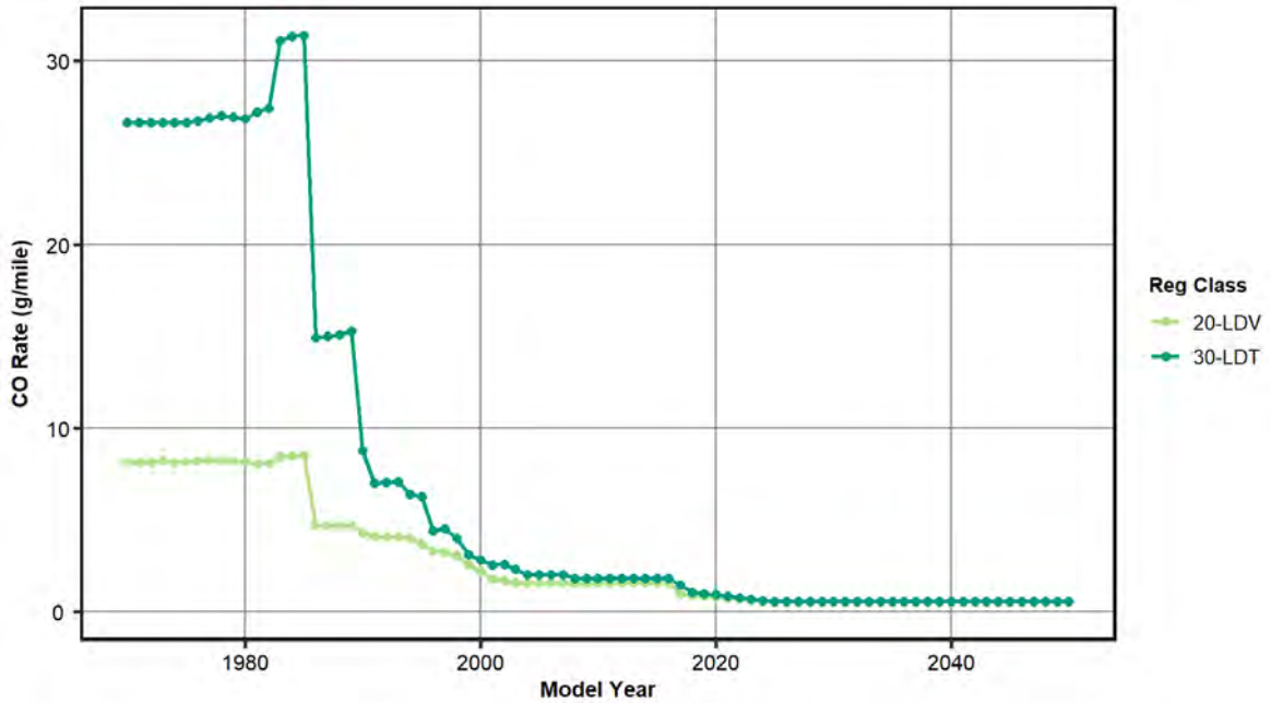
Figure 3-141 Base running emission rates for CO from age 0-3 gasoline light-duty vehicles averaged over a nationally representative operating mode distribution
