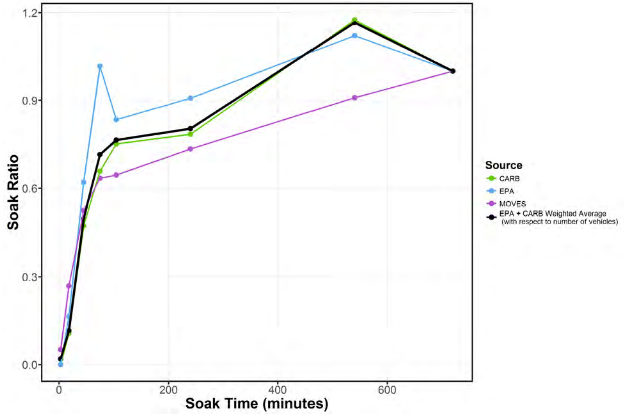
Figure 3-90 THC: Program-specific and final soak-time ratios for Tier-2/LEV-II vehicles. The “MOVES” line represents the values in MOVES for MY 2004 and later
