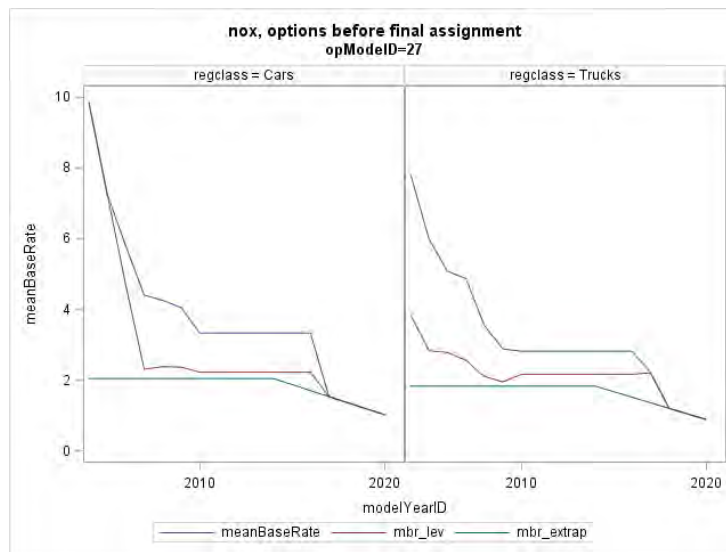
Figure 3-129 NO x : Trends in Emissions for Federal and Estimated CA/S.177 rates, for cars and trucks at age 0-3 years, for the running emissions process (opModelID = 27)
