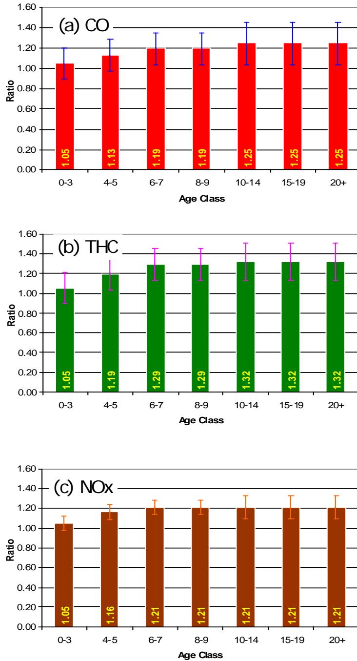
Figure 3-45 Final non-I/M ratios for 1990 and later model years for CO, THC and NO x , by MOVES ageGroups, with 95 percent confidence intervals
