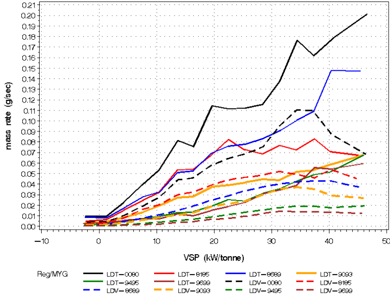
Figure 3-7 NO x emissions (g/sec) on aggressive cycles, vs. VSP, by regulatory class and model-year group
