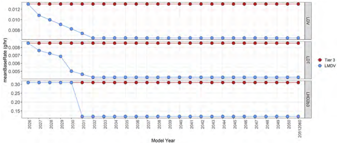
Figure 3-138 Comparison between Tier 3 rates and LMDV NO x rates for an example operating mode and age group for all regulatory classes affected by the LMDV rule.
