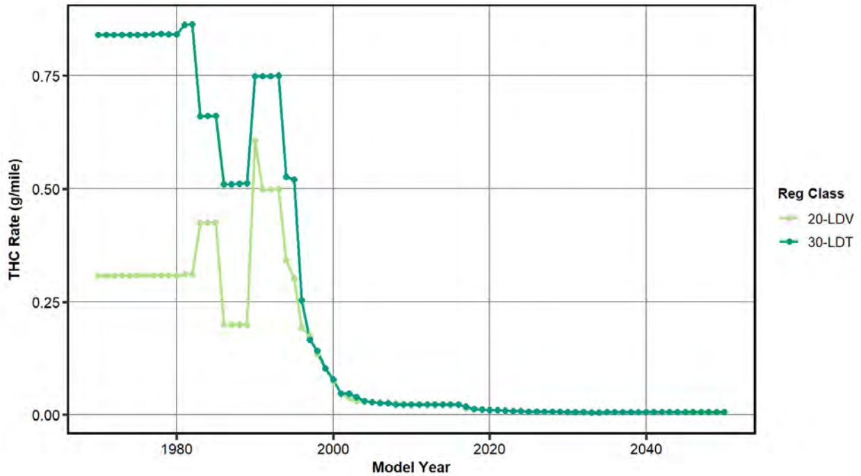
Figure 3-140 Base running emission rates for THC from age 0-3 gasoline light-duty vehicles averaged over a nationally representative operating mode distribution
