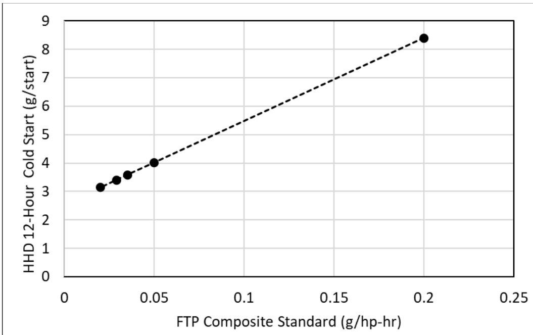
Figure 2-55 Calculated relationship between the HHD \text{NO}_x 12-hour cold-start and the composite FTP \text{NO}_x standards
