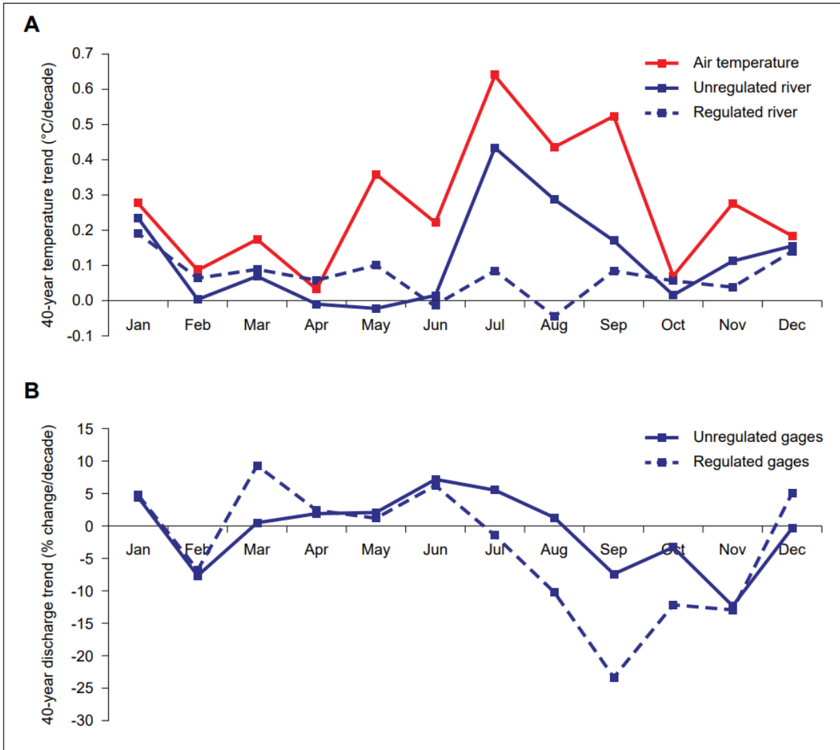
Figure 2-2: Trends in monthly mean air temperatures and river temperatures and discharge at long-term monitoring sites in the Southwest Oregon assessment area for the period 1976–2015. From USFS 2022b.
