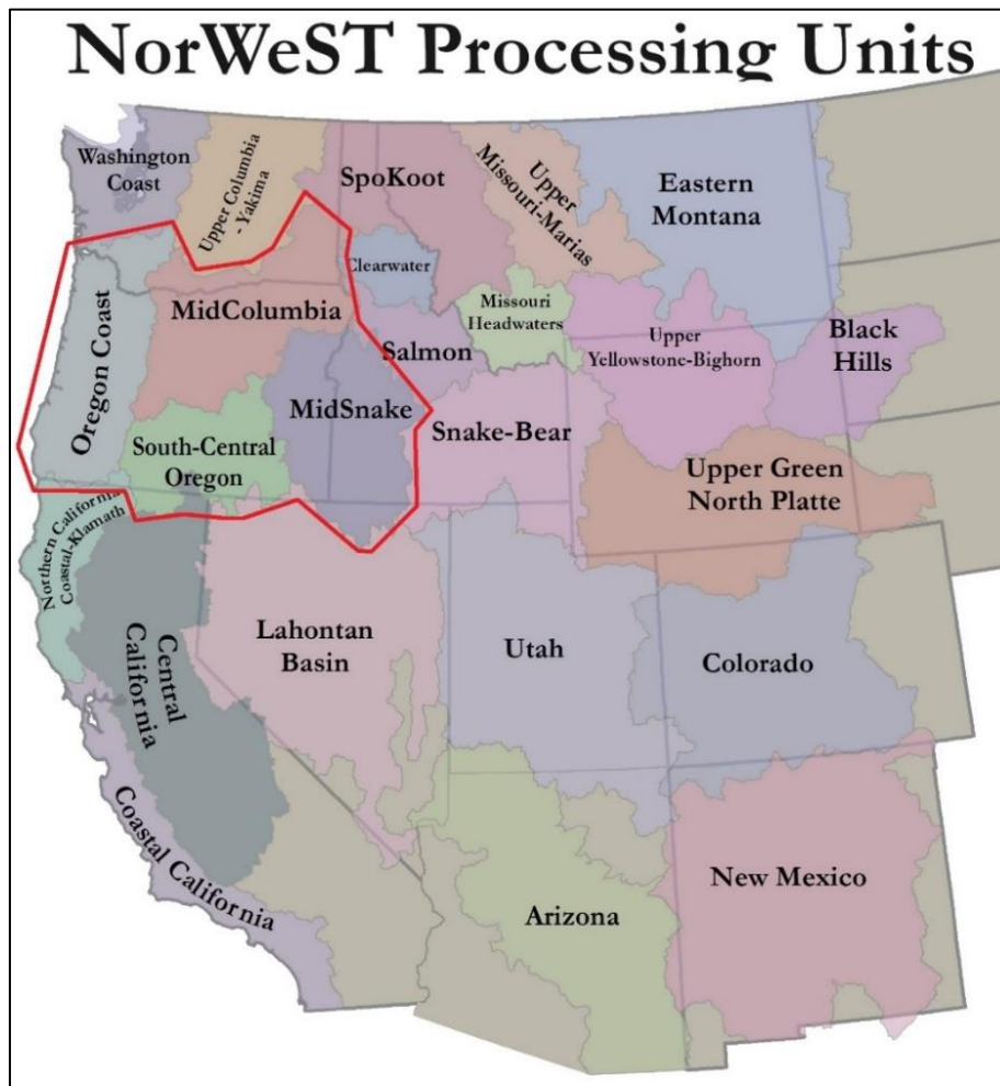
Figure 2-1: Map of NorWeST model area with Oregon-relevant processing units highlighted. Figure adapted from USFS (2022a).
