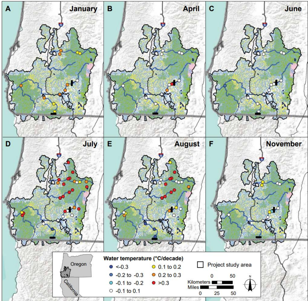
Figure 2-3: Decadal River temperature trends estimated from long-term monitoring records in the Southwest Oregon assessment area for the period 1976–2015. From USFS 2022b.
