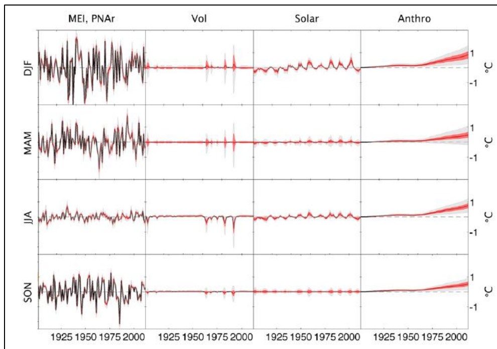
Figure 2-4: Drivers of air temperature in the Pacific Northwest during the 20th century. From Abatzoglou et al., 2014.
