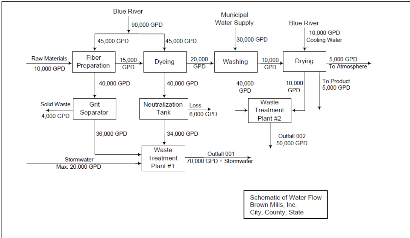
Exhibit 2C-1. Example Line Drawing
