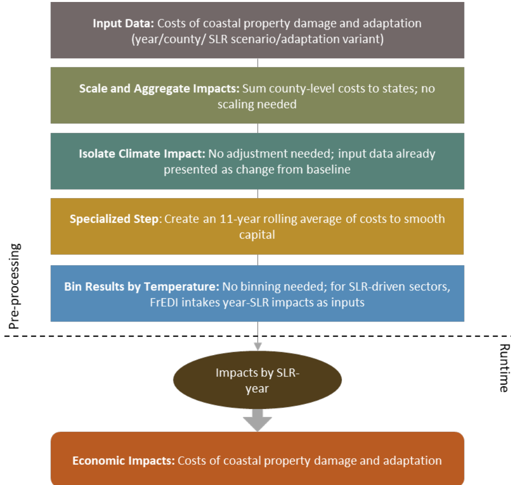
FIGURE B-23. COASTAL PROPERTIES DATA PROCESSING FRAMEWORK
