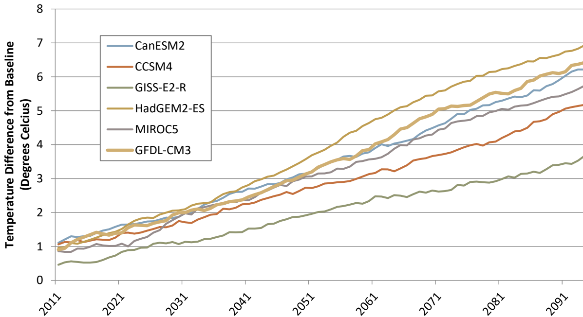
FIGURE C-3. CONUS DEGREES OF WARMING WITH 11-YEAR MOVING AVERAGE
