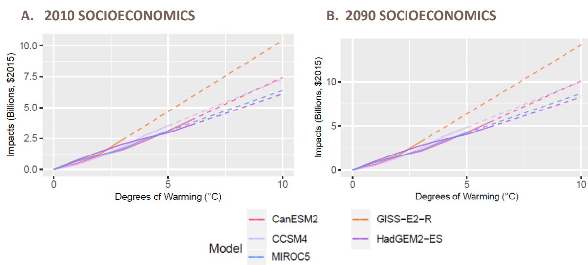
FIGURE B-42. WATER QUALITY IMPACTS BY TEMPERATURE BIN DEGREE
