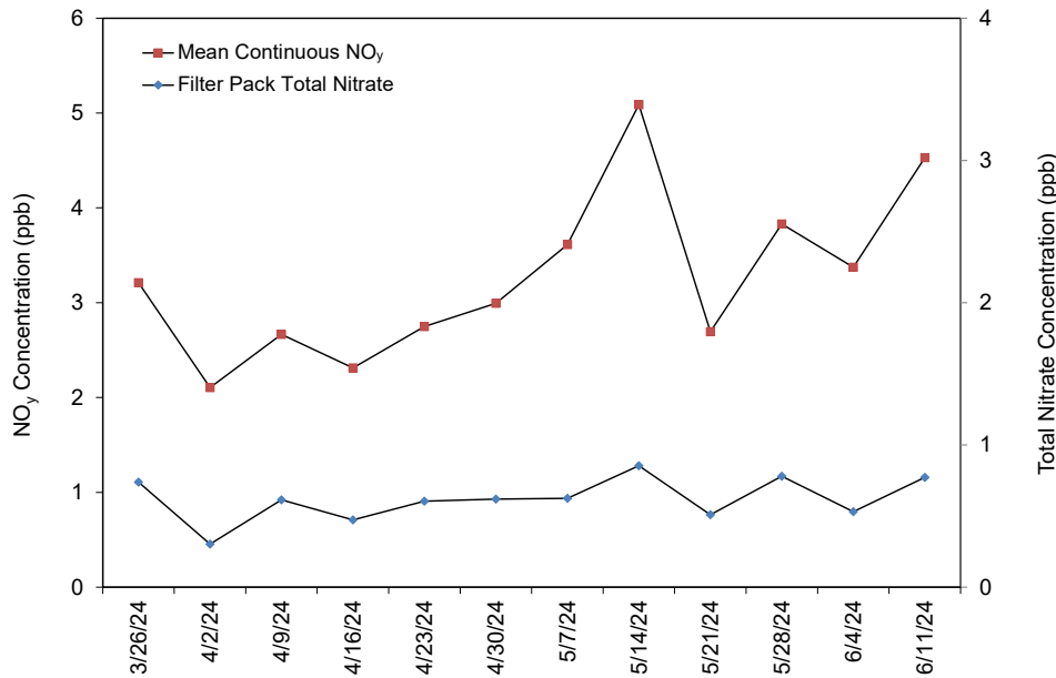
Figure 30. Comparison of BVL130, IL Weekly Mean Continuous NO y and Total NO 3 Concentrations
