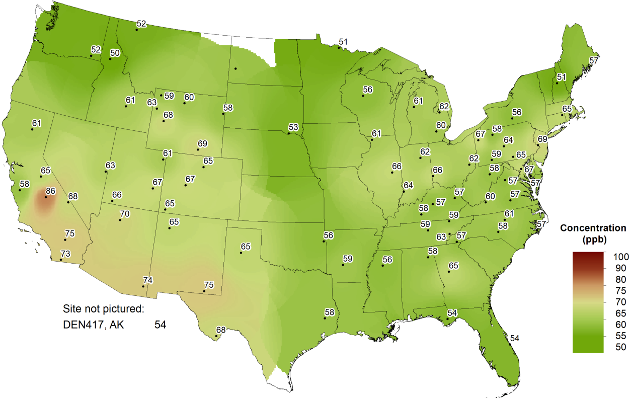
Figure 1. Fourth Highest Daily Maximum 8-hour Average O 3 Concentrations (ppb) through Second Quarter 2024
