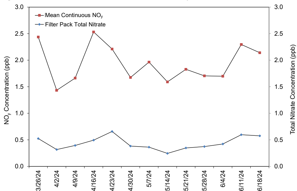
Figure 29. Comparison of DUK008, NC Weekly Mean Continuous NO y and Total NO 3 Concentrations
