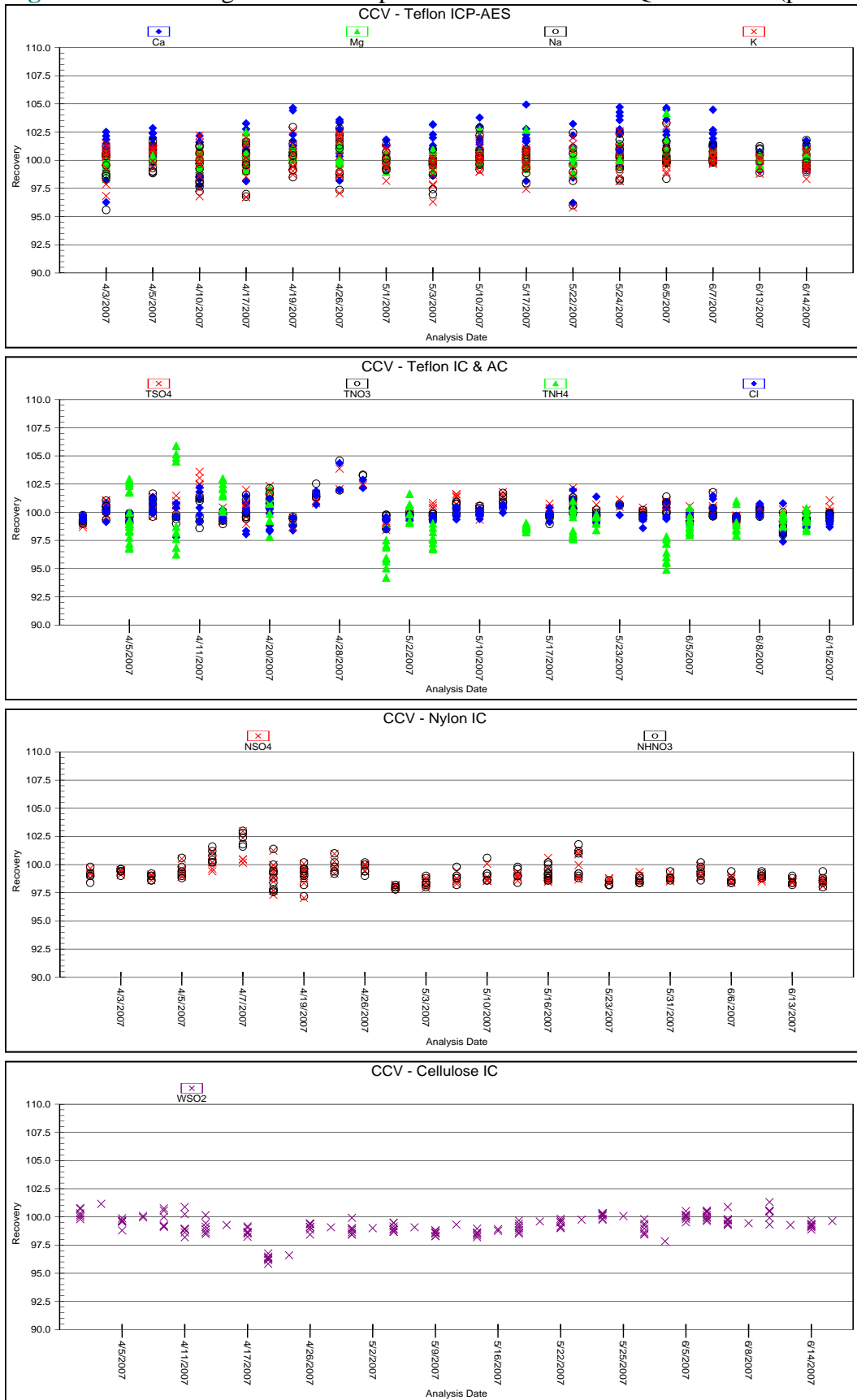
Figure 2. Continuing Calibration Spike Results for Second Quarter 2007 (percent recovery)
