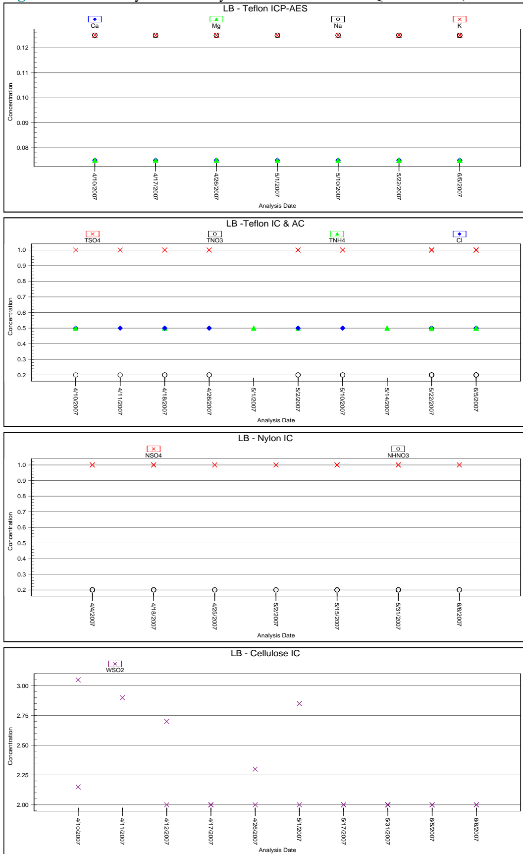
Figure 7. Laboratory Blank Analysis Results for Second Quarter 2007 (total micrograms)
