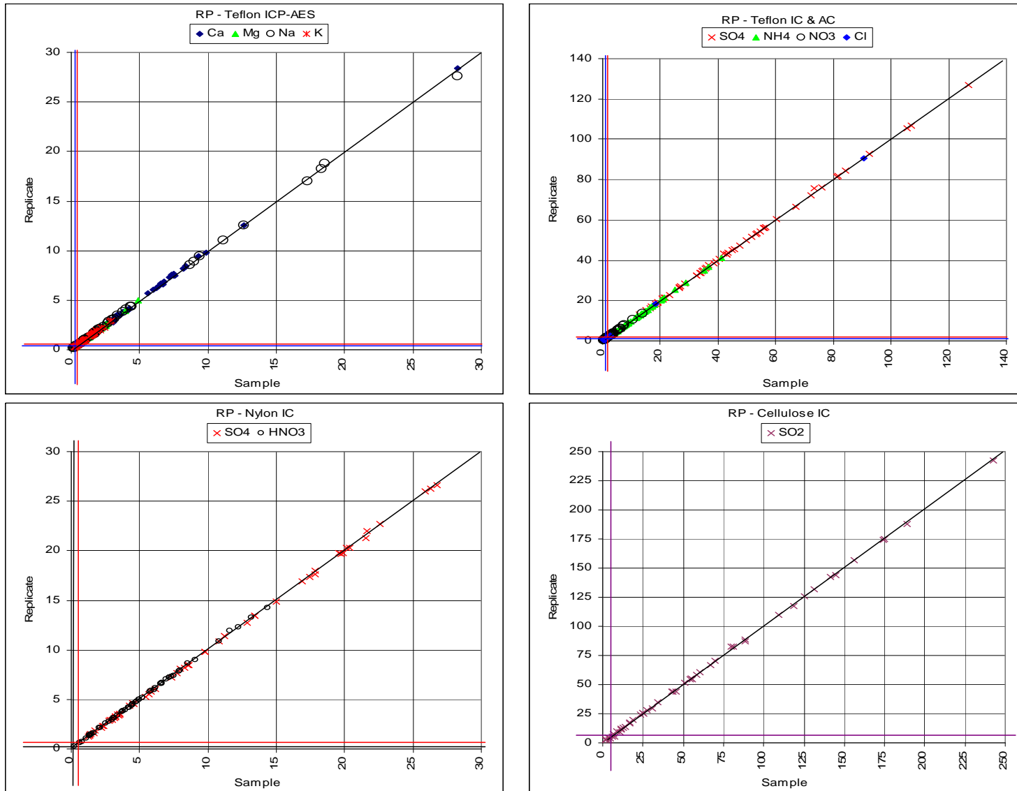
Figure 3. Replicate Sample Analysis Results for Second Quarter 2007 (total micrograms)
