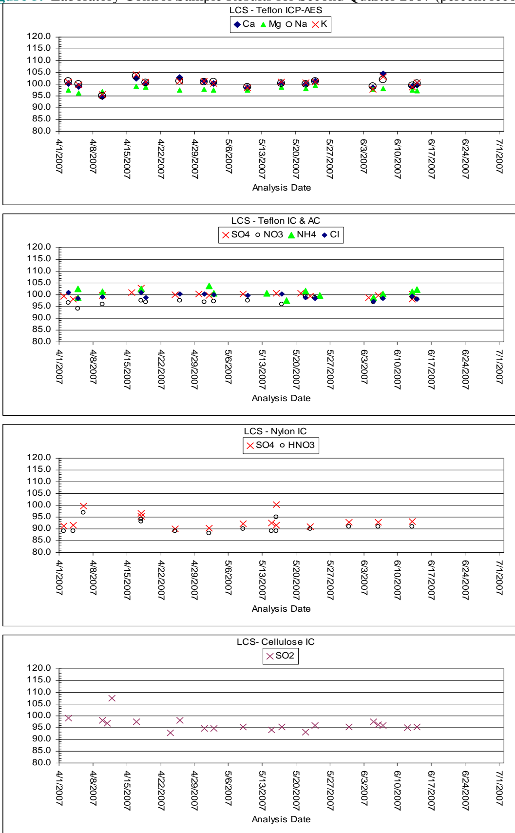
Figure 5. Laboratory Control Sample Results for Second Quarter 2007 (percent recovery)
