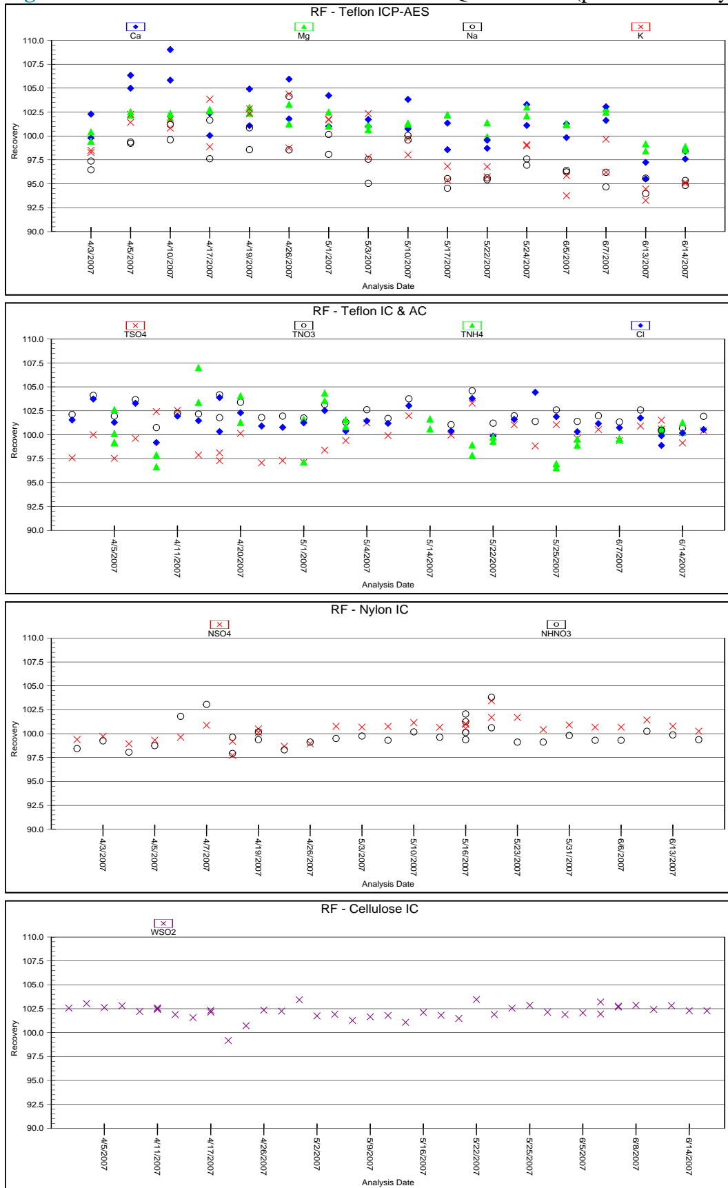
Figure 1. Reference Standard Results for Second Quarter 2007 (percent recovery)
