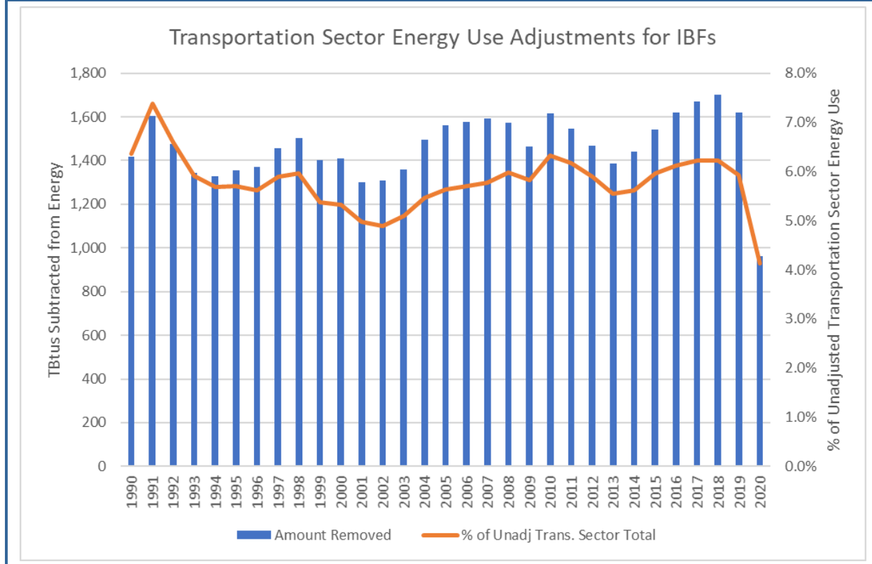
Figure 2-11: Adjustments Made to Transportation Sector Energy Use to Account for IBFs
