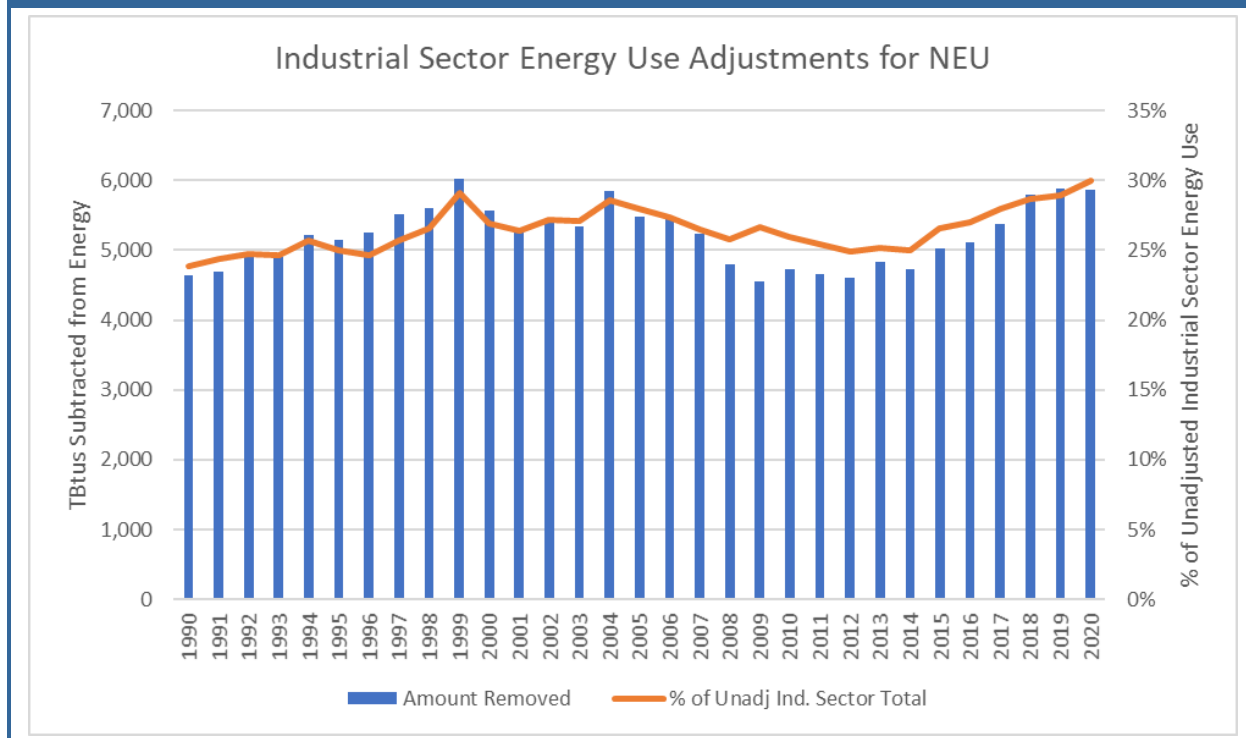
Figure 2-10: Adjustments Made to Industrial Sector Energy Use to Account for Emissions Reported as NEUs
