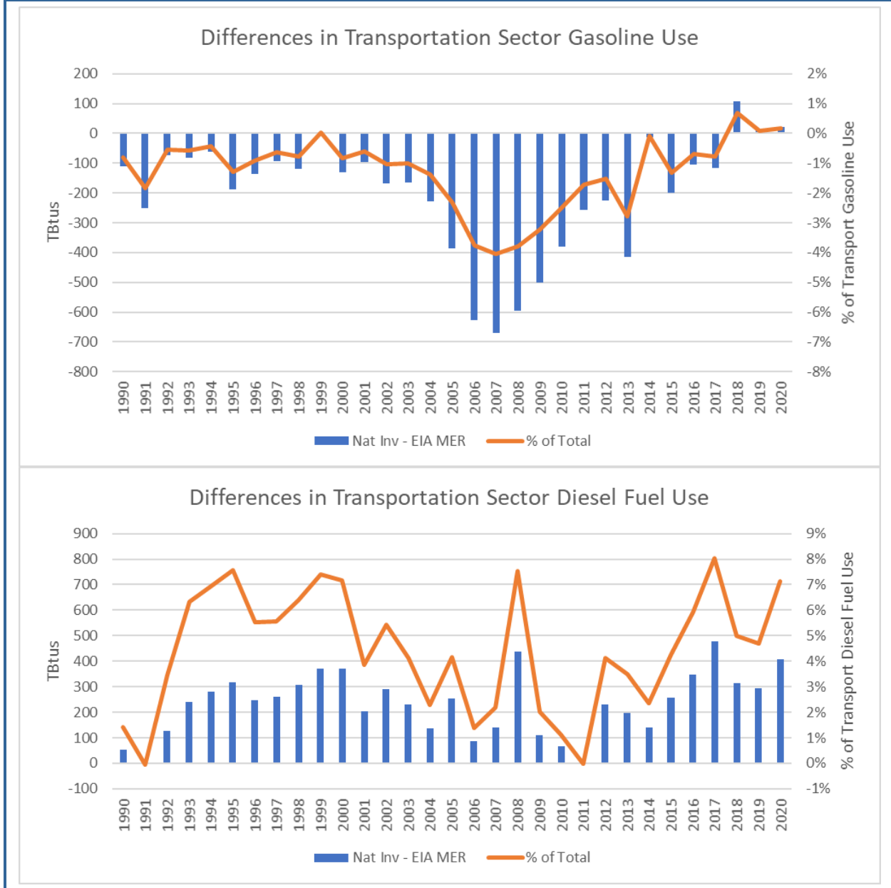
Figure 2-8: Comparison of Transportation Sector Fuel Use
