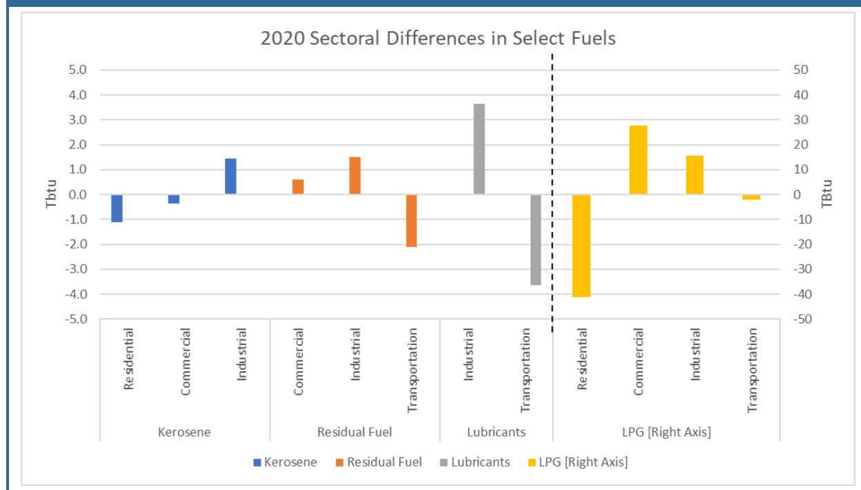
Figure 2-4: 2020 Differences Between Sectors for Petroleum Fuels (SEDS—National Inventory )
