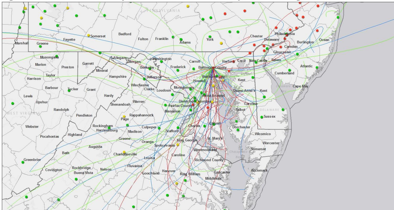
Figure 7a. HYSPLIT Back Trajectories for Baltimore County, MD Violating Monitor 240051007 a .
