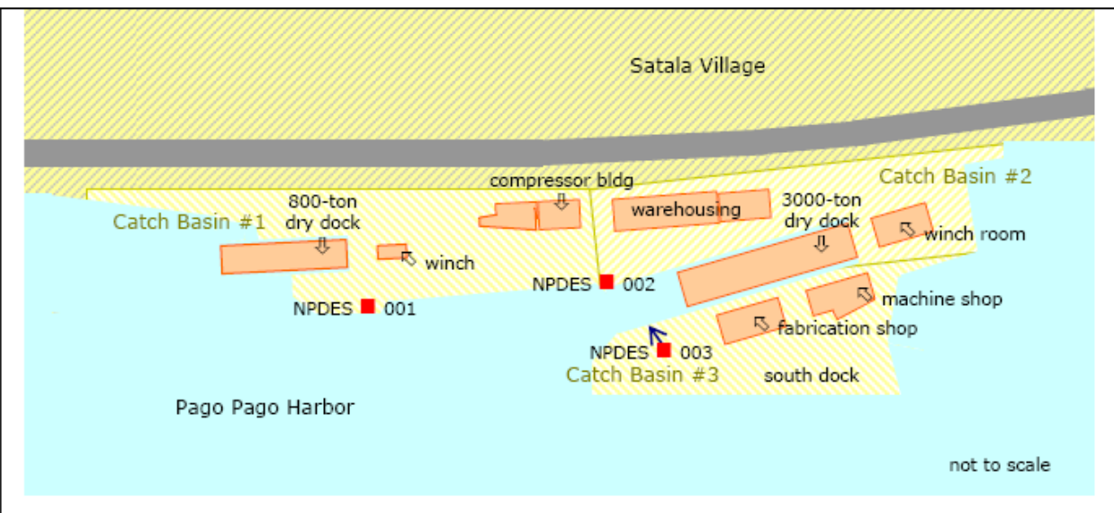
Figure 1. MYD Samoa Shipyard – Layout map with major structures and existing NPDES discharge points indicated.
