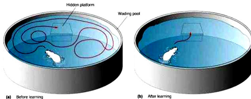
Figure 2. Morris Water Maze. Animals must navigate a large pool to find a hidden escape platform submerged below the water surface. Different starting points are used on each trial but the position of the platform remains fixed over trials. Distal cues are placed on the walls surrounding the maze and remain invariant over the course of the training.
