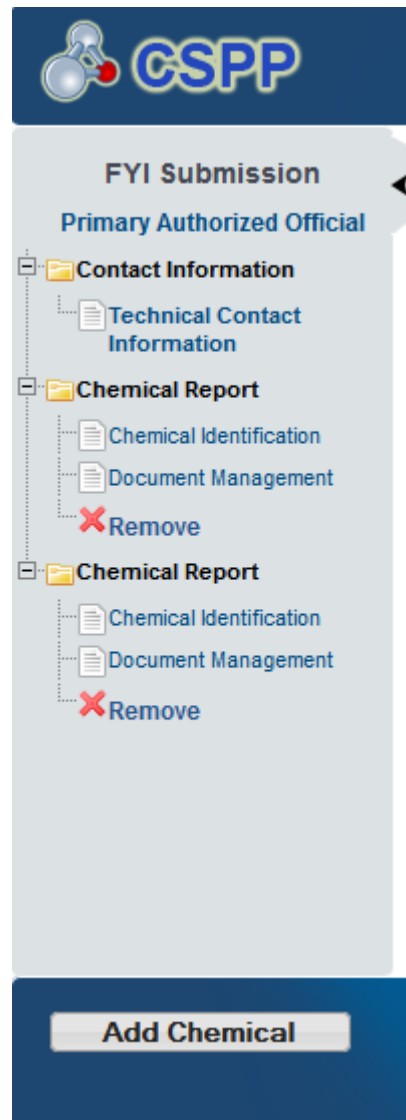
Exhibit 3-8: Navigation Tree
