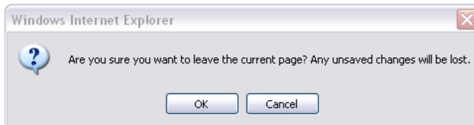
Exhibit 3-7: Navigation Prompt
