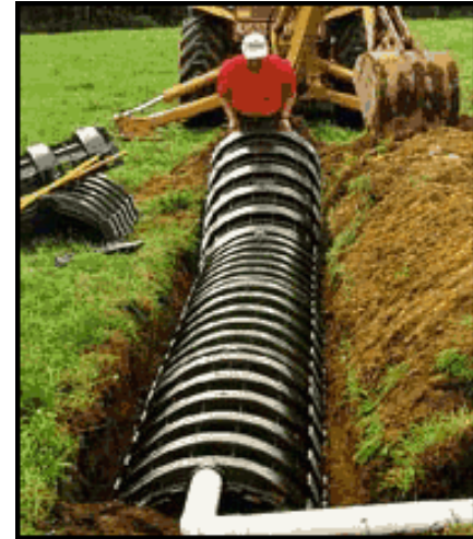
FIGURE 1 LEACHING CHAMBER
