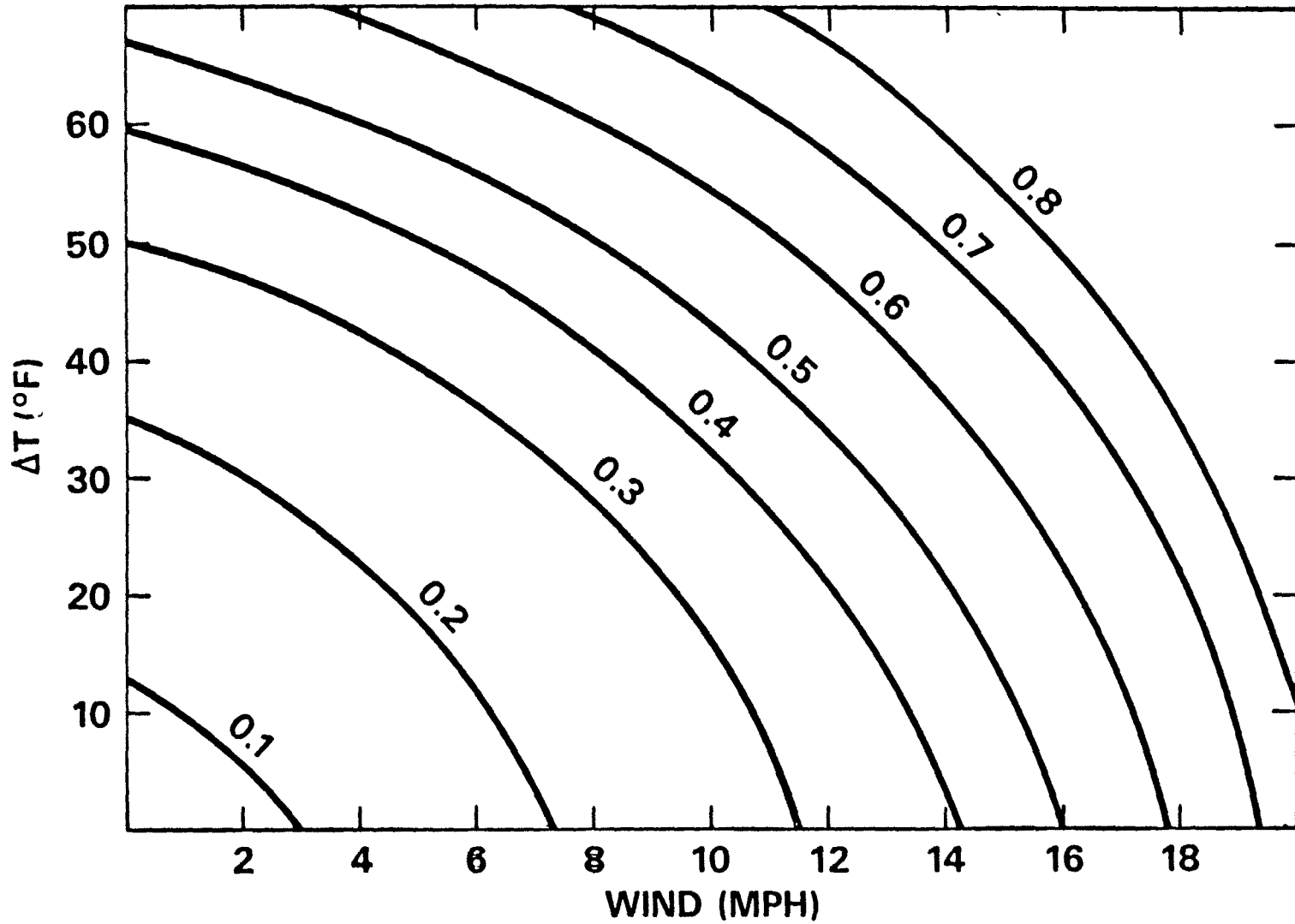
Fig. 1 Exchange rate for closed homes of modern construction and good insulation, with furnace and fans off. The number of air exchanges per hour are presented as a function of the indoor-outdoor temperature difference and the wind speed.
