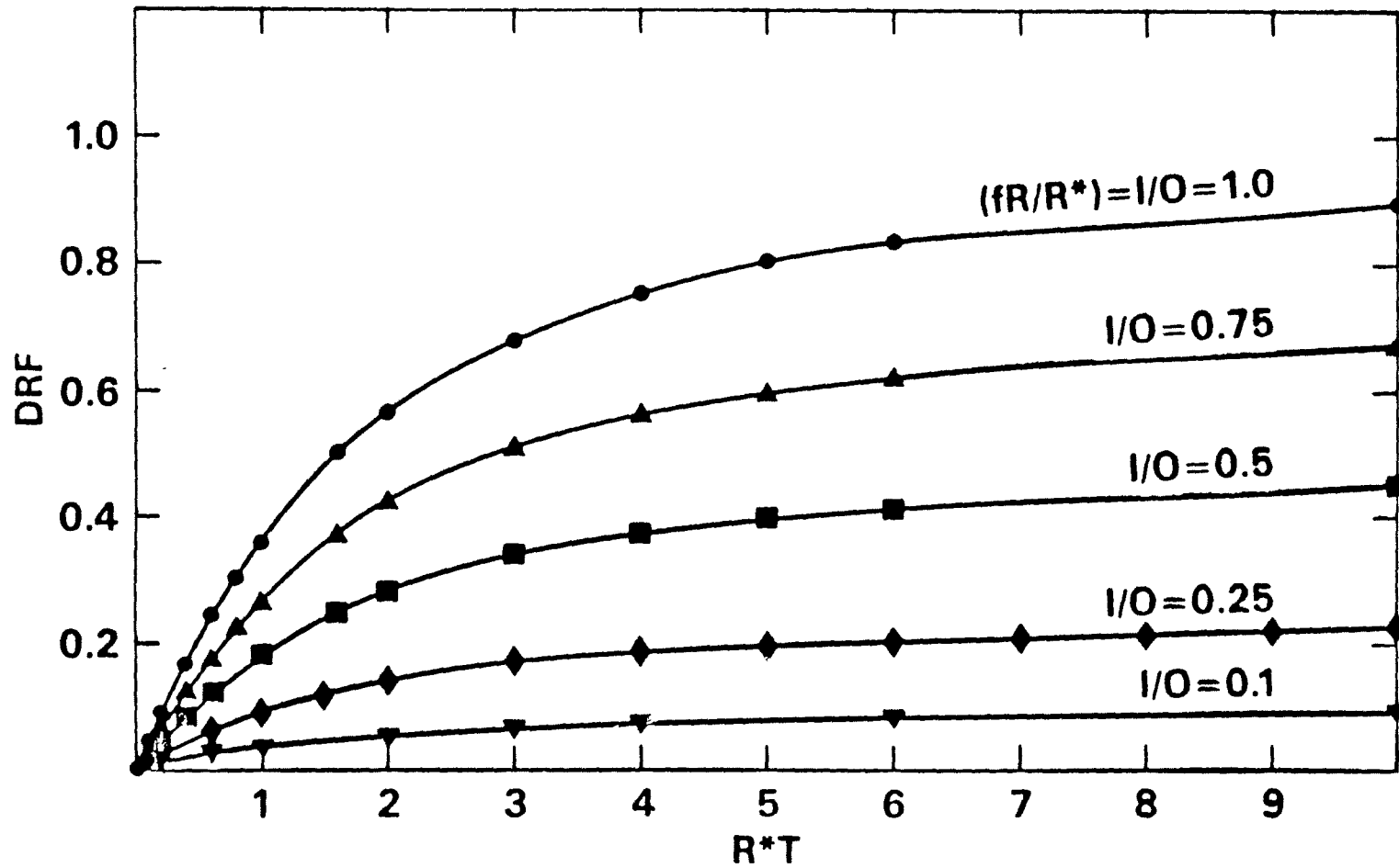
Fig. 3 The Dose Reduction Factor (DRF) as a function of the air exchange rate, R , time, T , fraction of the contaminant that penetrates the shelter's structure, f , and the virtual air exchange rate, R^* . At large values of R^*T , the DRF approaches the equilibrium ratio of indoor and outdoor concentrations, I/O .
