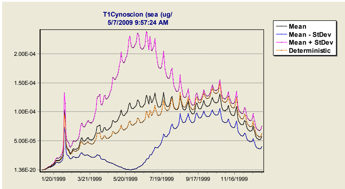
Figure 65. Sensitivity of concentration of PCBs in sea trout as a function of sea trout T Opt in Galveston Bay TX.
