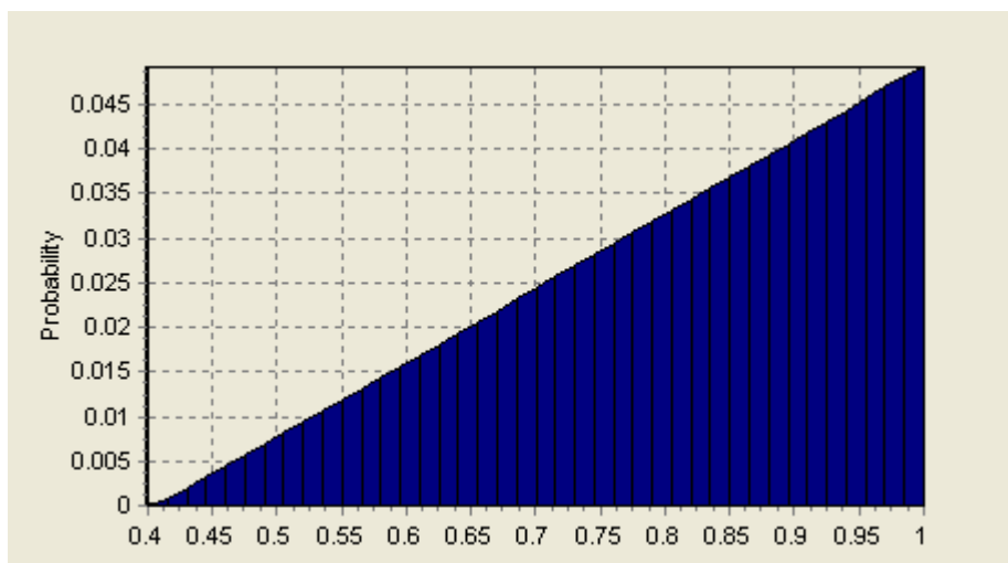
Figure 50. Skewed triangular distribution of selective sorting used in analysis.
