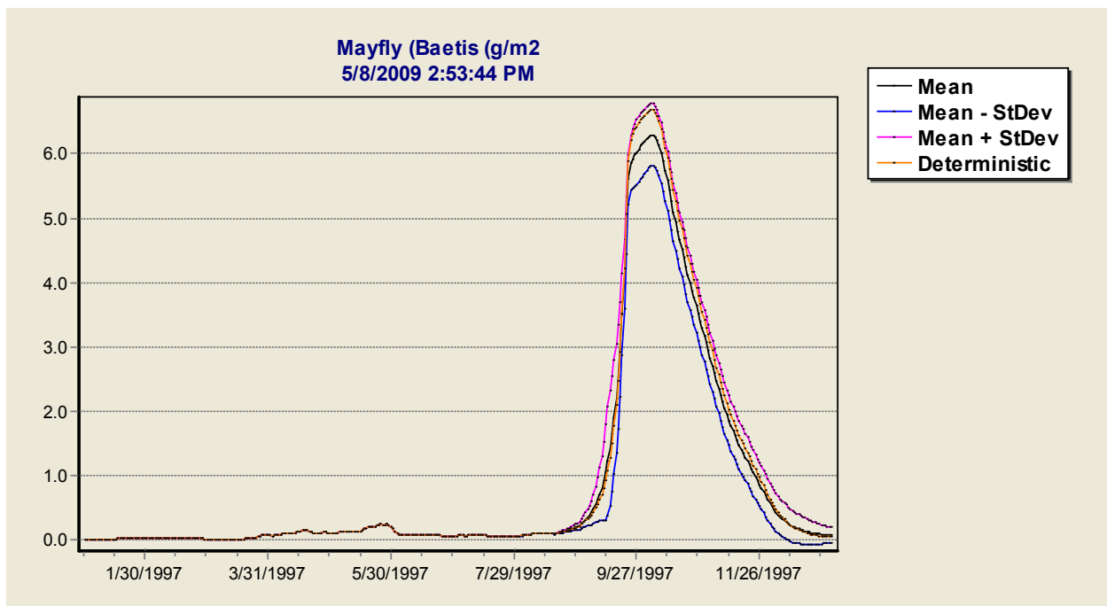
Figure 62. Sensitivity of mayflies in Ohio stream to yellow perch LC50.
