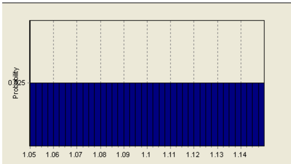
Figure 40. Distribution of Theta for refractory particulate organic carbon.
