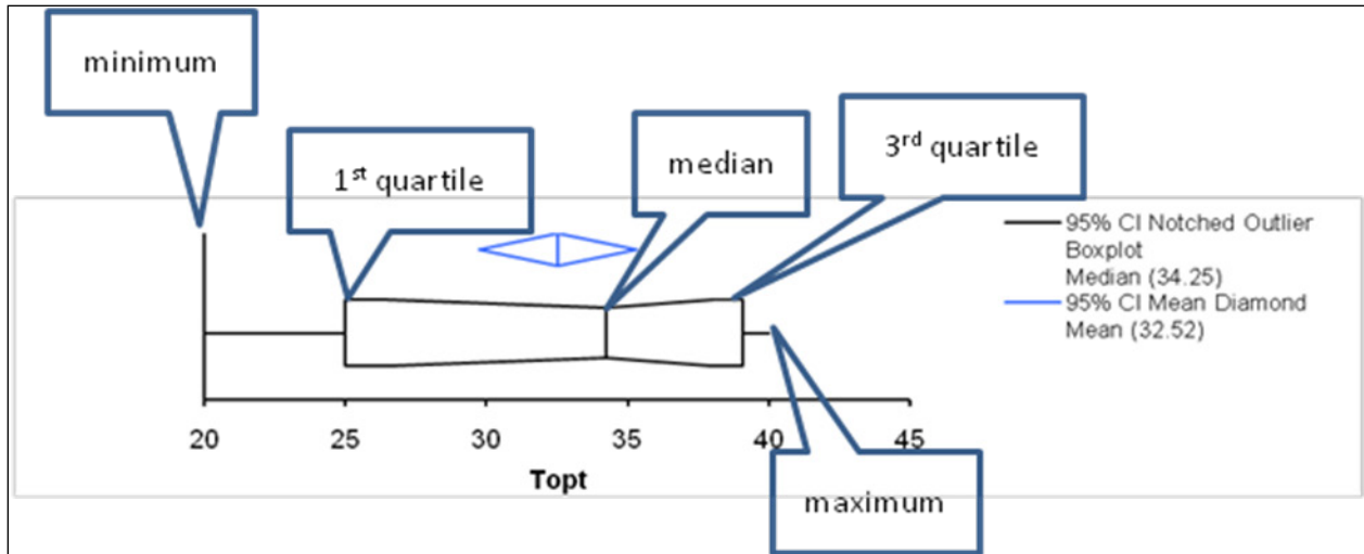
Figure 30. Box and whisker plot of observed blue-green TOpt values.
