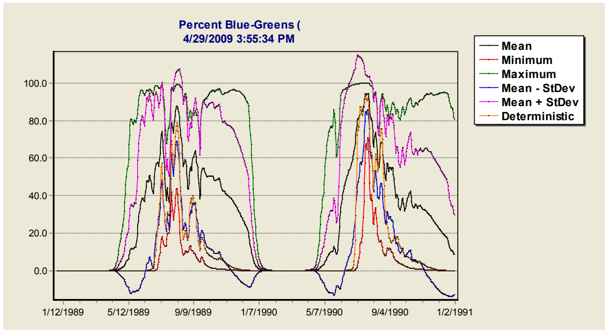
Figure 31. Sensitivity of percent blue-greens to blue-green TO_{opt} in Onondaga Lake NY.
