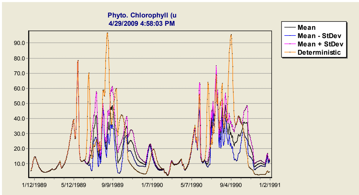
Figure 37. Sensitivity of chlorophyll a to diatom PMax in Lake Onondaga NY.
