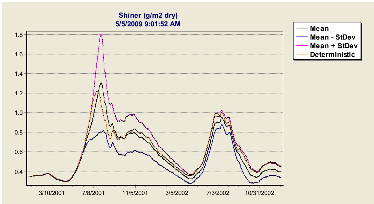
Figure 45. Sensitivity of shiners to smallmouth bass TOpt in Cahaba River AL.
