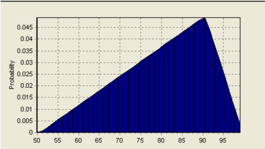
Figure 47. Triangular distribution of percent lost with sloughing used in analysis.
