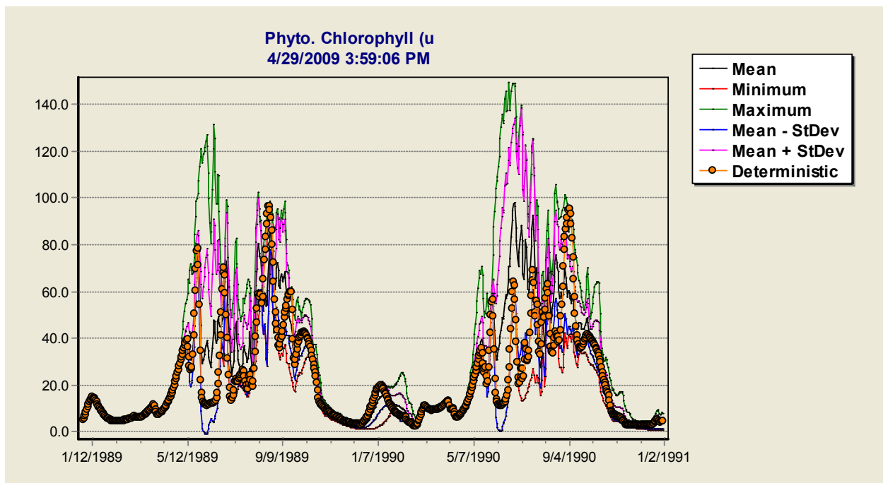
Figure 32. Sensitivity of chlorophyll a to blue-green TO_{opt} in Onondaga Lake NY.
