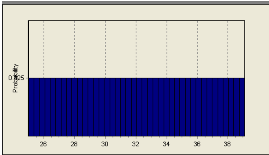
Figure 29. Distribution of blue-green TOpt values used in analysis.
