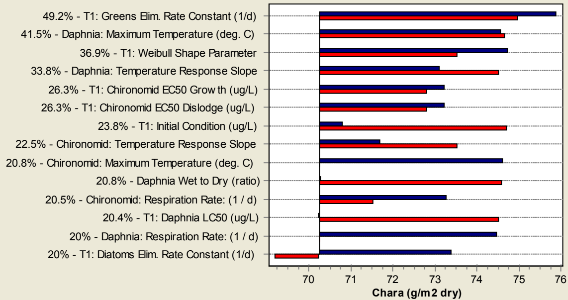
Figure B-19: Duluth Pond, Chara, 15% parameter test.
