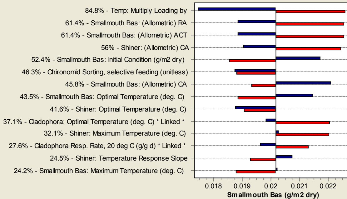
Figure B-15: Cahaba River, Smallmouth Bass, YOY.
