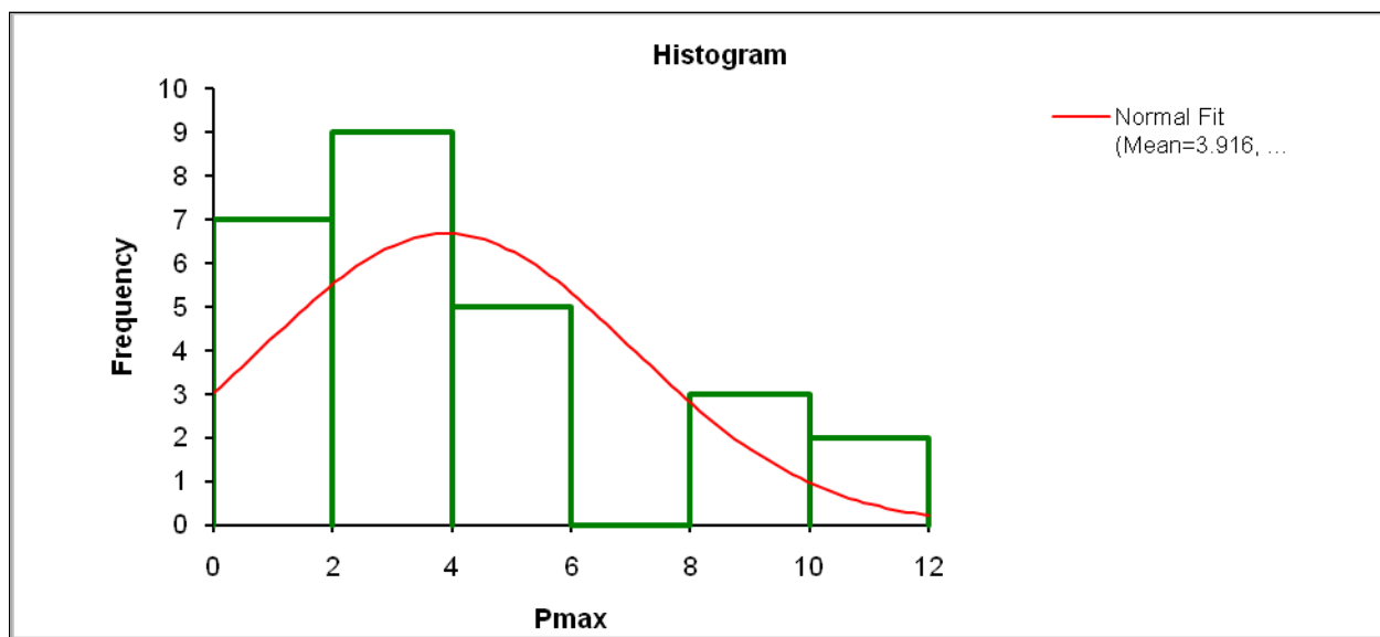
Figure 22. Histogram of observed Blue-Green P Max values from Collins and Wlosinski (1983).
