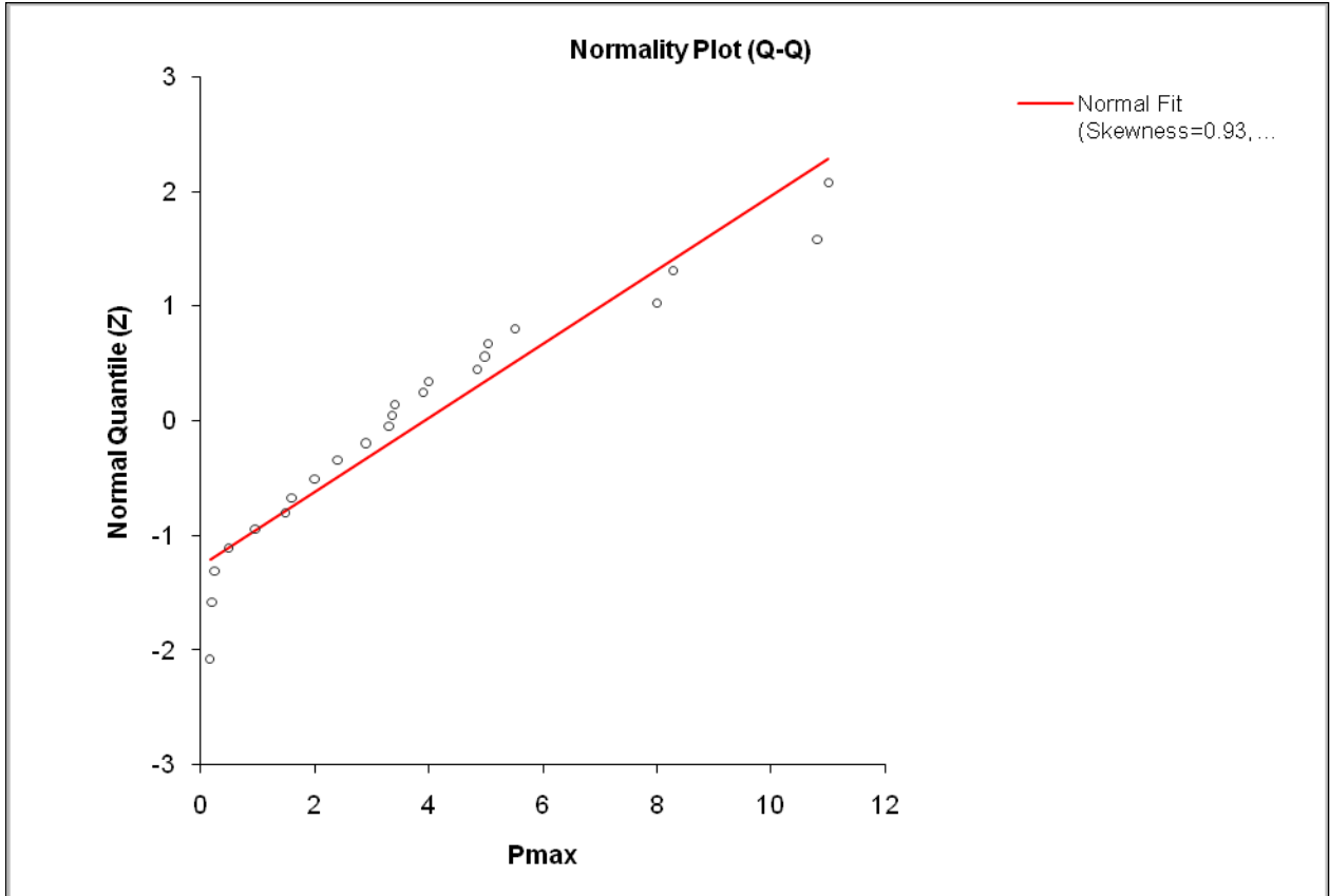
Figure 23. Normality of observed blue-green PMax values from Collins and Wlosinski (1983).
