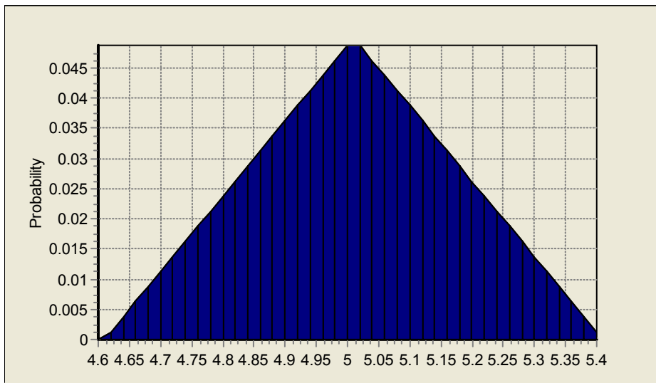
Figure 53. Triangular distribution of log K_{ow} for chlorpyrifos used in analysis.
