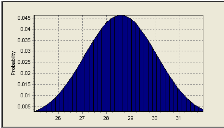
Figure 43. Distribution of smallmouth bass TOpt values used in analysis.
