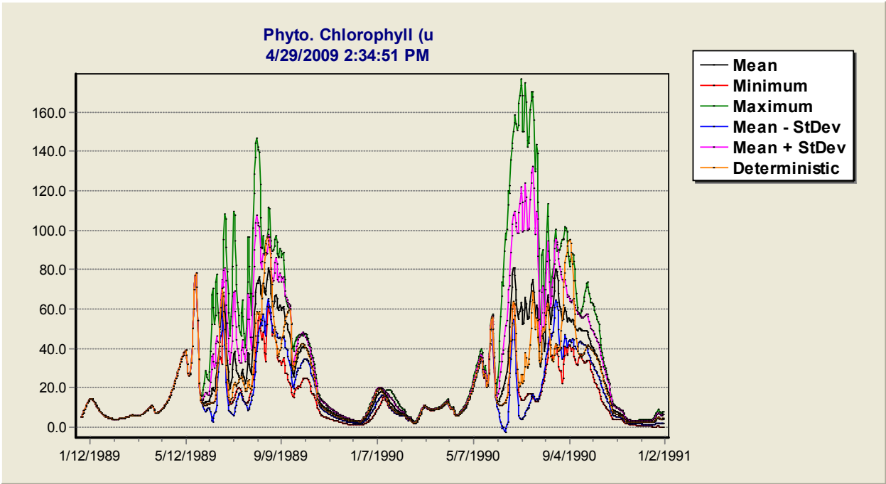
Figure 27. Sensitivity of chlorophyll a to blue-green PMax in Onondaga Lake NY.
