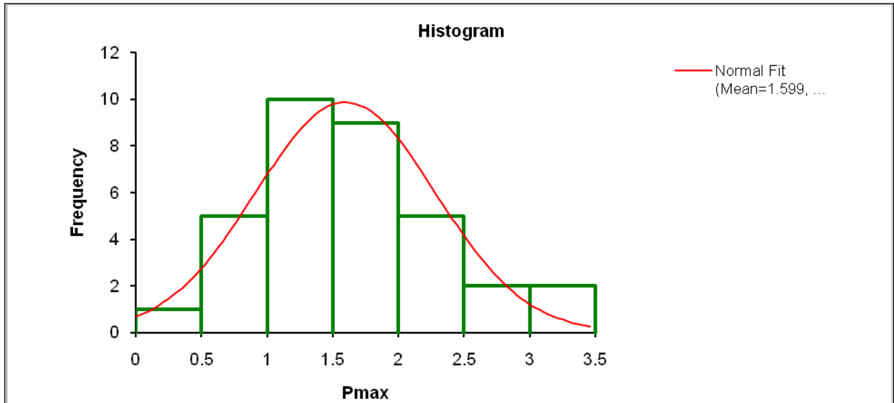
Figure 33. Histogram of observed diatom P_{Max} values.
